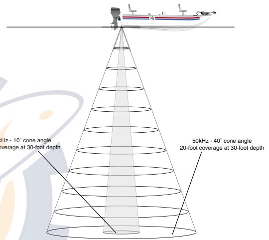
Transducer coverage
